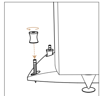
4 Secure their adjustment with the nuts provided.
