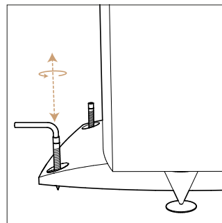
3 Using the key provided, adjust the flatness while decoupling your speaker from the floor by a few millimeters.
